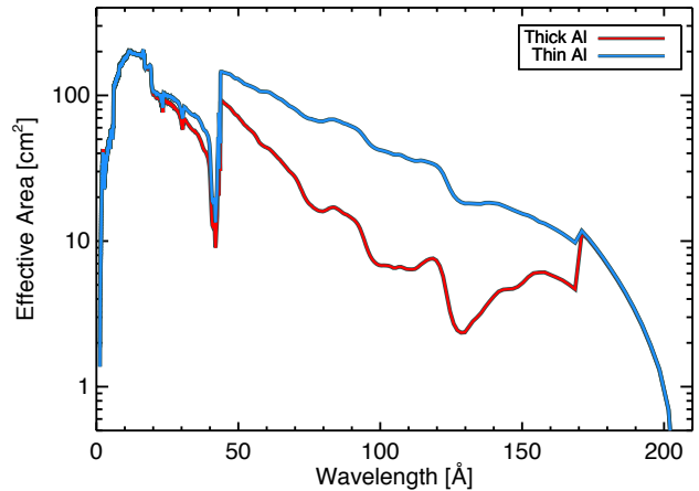
Figure 2. The effective areas of the Chandra HRC-S “thin” and “thick” Al filter regions computed at the location of the region boundary in the -y direction from the detector centre.
