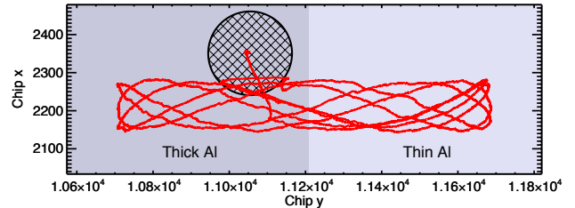
Figure 3. The dither pattern followed by LHS 248 in HRC-S detector coordinates. The hashed circle represents the size of the converging light cone at the height of the UVIS above the focal plane and is centred on the acquisition position of the target at the beginning of the observation. Note that the detector Chip\ y coordinate is oriented in the opposite direction to the spacecraft coordinates noted in Figure 1.
