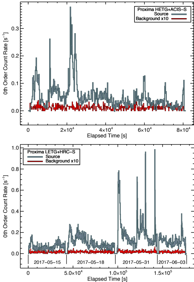
Figure 8. X-ray light curves of Proxima observed with the Chandra HETG+ACIS-S (top), and LETG+HRC-S (bottom). Light curves were obtained from the 0th orders in both cases, and were binned at intervals of 200s. The HETG+ACIS-S 0th order light curve has been corrected for pile-up (see text).
