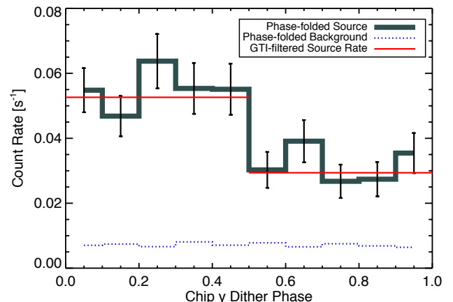
Figure 6. Source and background count rates as a function of the Chip y dither phase excluding the large flare toward the end of the observation. The mean count rates for the exclusively thick or thin “good time intervals”, for which the times during which the source was crossing the thick/thin boundary have been filtered out, are also indicated.
