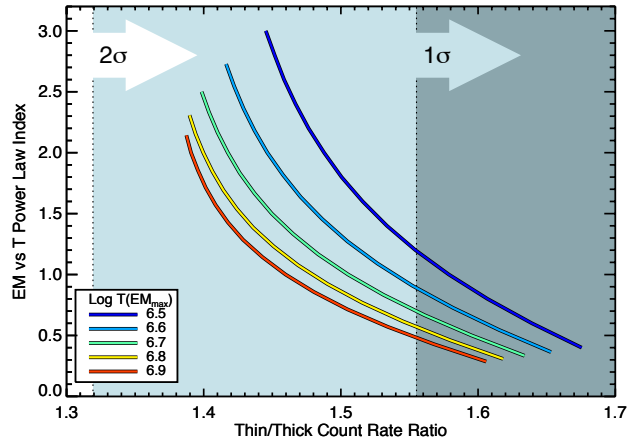
Figure 12. Loci of the EMD power law index as a function of model thin/thick filter count rate ratio. The 1\sigma and 2\sigma lower limits to the observed ratio of 1.79 \pm 0.24 for LHS 248 are indicated.
