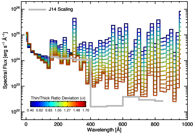
Figure 13. Synthetic spectra computed from the model DEMs with \log T_{peak} = 6.5 for inverse FIP abundances binned on 20 Å intervals and colour-coded according to the deviation in their predicted thin/thick filter ratios from the observed LHS 248 value. The flux predicted by the Linsky et al. (2014) empirical scaling based on the Ly \alpha flux of Proxima, scaled to the radius of LHS 248 is also shown (denoted J14).
