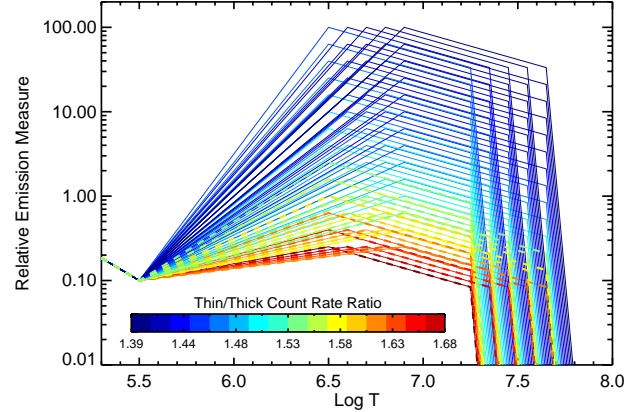
Figure 11. The idealised set of DEMs investigated for LHS 248 in this study colour-coded according to their corresponding Thin/Thick predicted count rate ratio. Models that yielded a ratio in agreement with the observed value at the 1\sigma level are shown overlaid with bold dashed lines.
