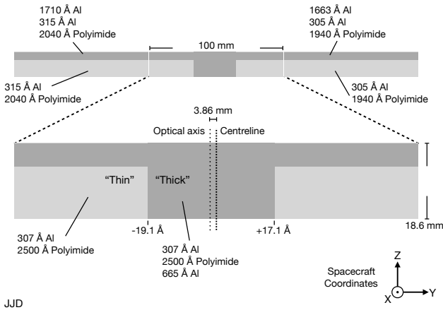
Figure 1. A schematic of the Chandra HRC-S UV/Ion shield with the centre segment shown enlarged for detail. The filter characteristics of the “thin” and “thick” Al regions of the central segment referred to and used in the observations described here are noted. The observation of LHS 248 was obtained by pointing 5.03 arcmin in the positive y direction so as to place the source at the thick/thin Al filter boundary in the -y direction, to the left of centre as shown here.
