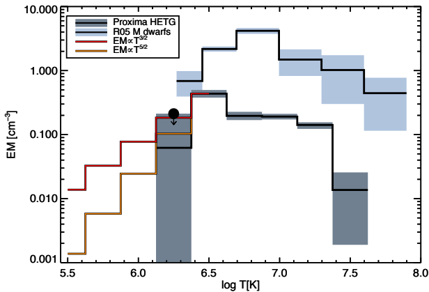
Figure 10. Emission measure distributions derived from HETG+ACIS-S observations of Proxima, together with the mean DEM from the XMM-Newton M dwarf study of Robrade & Schmitt (2005, R05) . The grey shaded regions represent uncertainties in the form of 90% confidence intervals. The cool extensions of the Proxima DEM tested on the LETG+HRC-S spectrum of Proxima are also illustrated.
