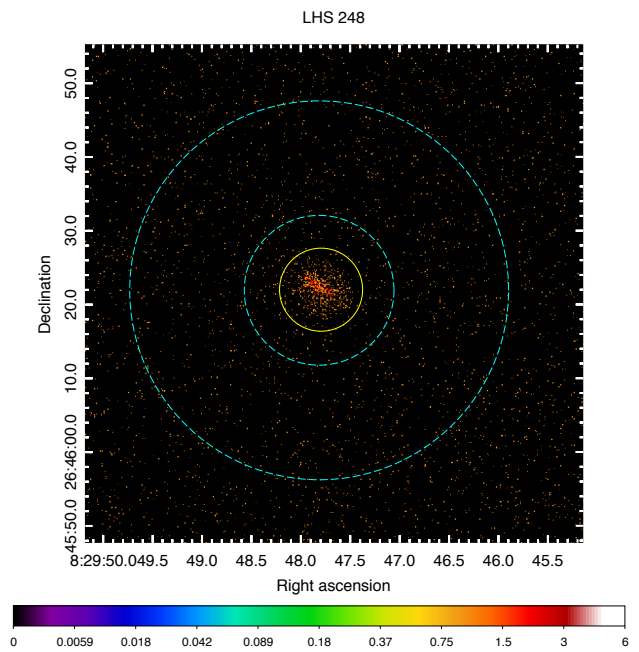
Figure 4. HRC-S image of LHS 248 in sky coordinates illustrating the source and background signal extraction regions employed in the analysis. The asymmetric nature of the distribution of photon counts is a result of the source being observed off-axis.
