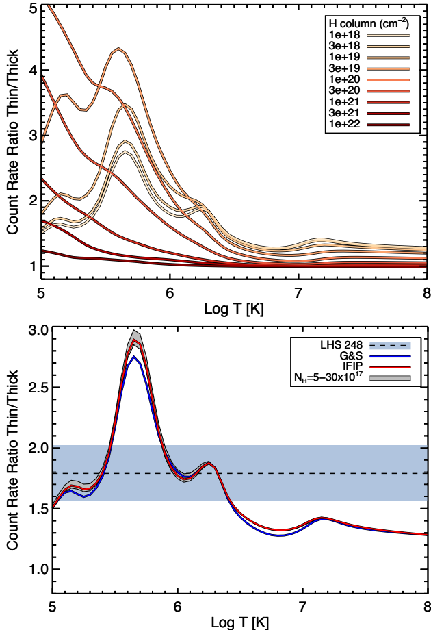
Figure 7. The predicted thin/thick filter count rate ratio for isothermal optically-thin plasma radiative loss models. Top: for the solar (Grevesse & Sauval 1998) abundance mixture and different values of interstellar medium neutral hydrogen column density. Bottom: The count rate ratio for the column density range appropriate to LHS 248, and including both solar (“G&S”) and inverse FIP (see text) abundance mixtures; the observed ratio for LHS 248 is also indicated.
