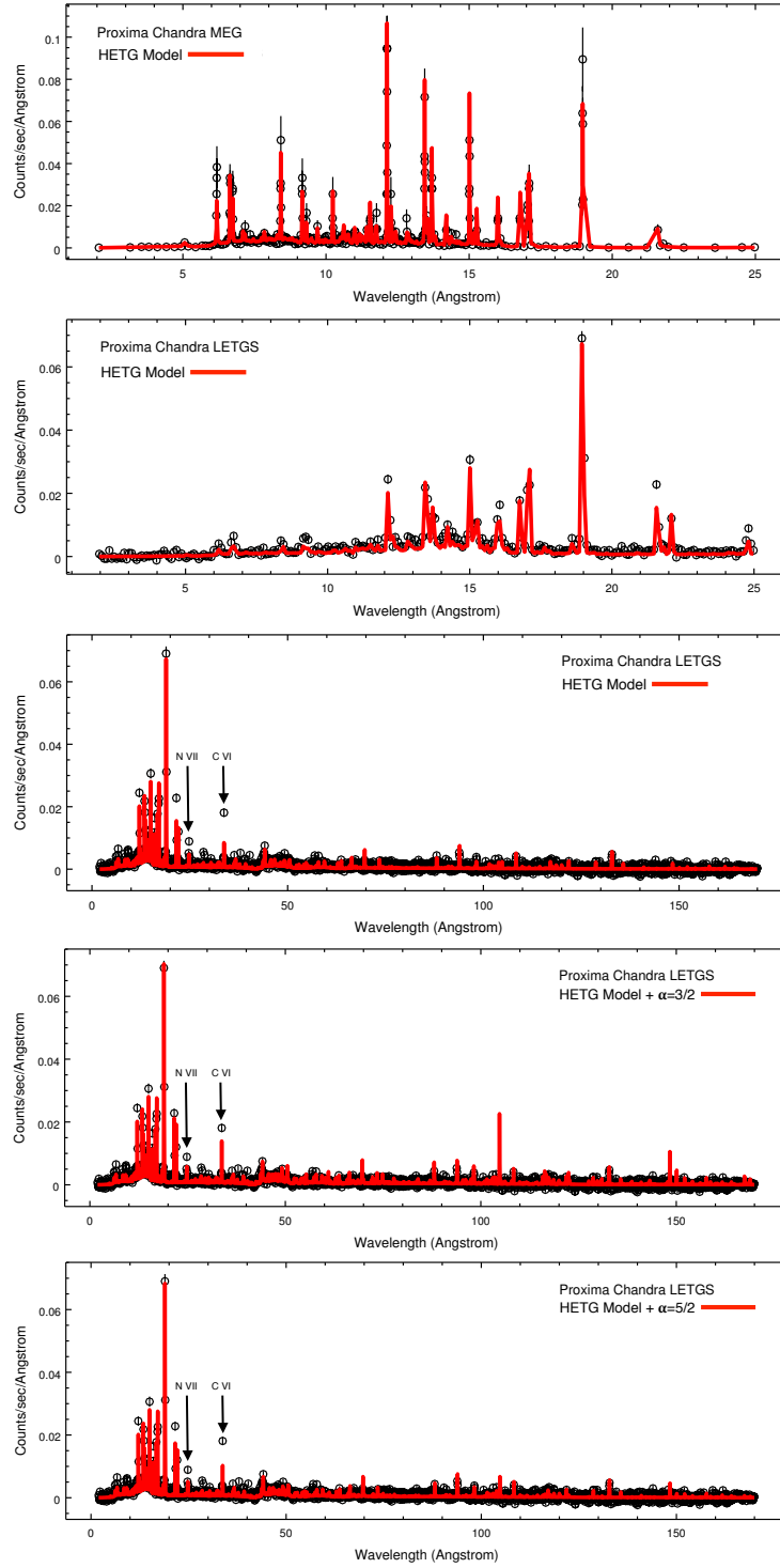
Figure 9. The Chandra HETG (top panel) and LETG (lower four panels) spectra of Proxima overlaid with the best-fit HETG model spectrum (see text for details). The lower three panels illustrate the full range of the LETG+HRC-S spectrum and show the effect of changing the cool “tail” of the DEM. The first of these (middle panel) illustrates the HETG model with no additional cool plasma components. The lower two show the HETG model augmented by cool DEM extensions that follow the power law relation DEM(T) \propto T^\alpha with \alpha = 3/2 (fourth panel down) and \alpha = 5/2 (bottom panel). In order to aid the visualizations of the model comparisons, spectra have been rebinned.
