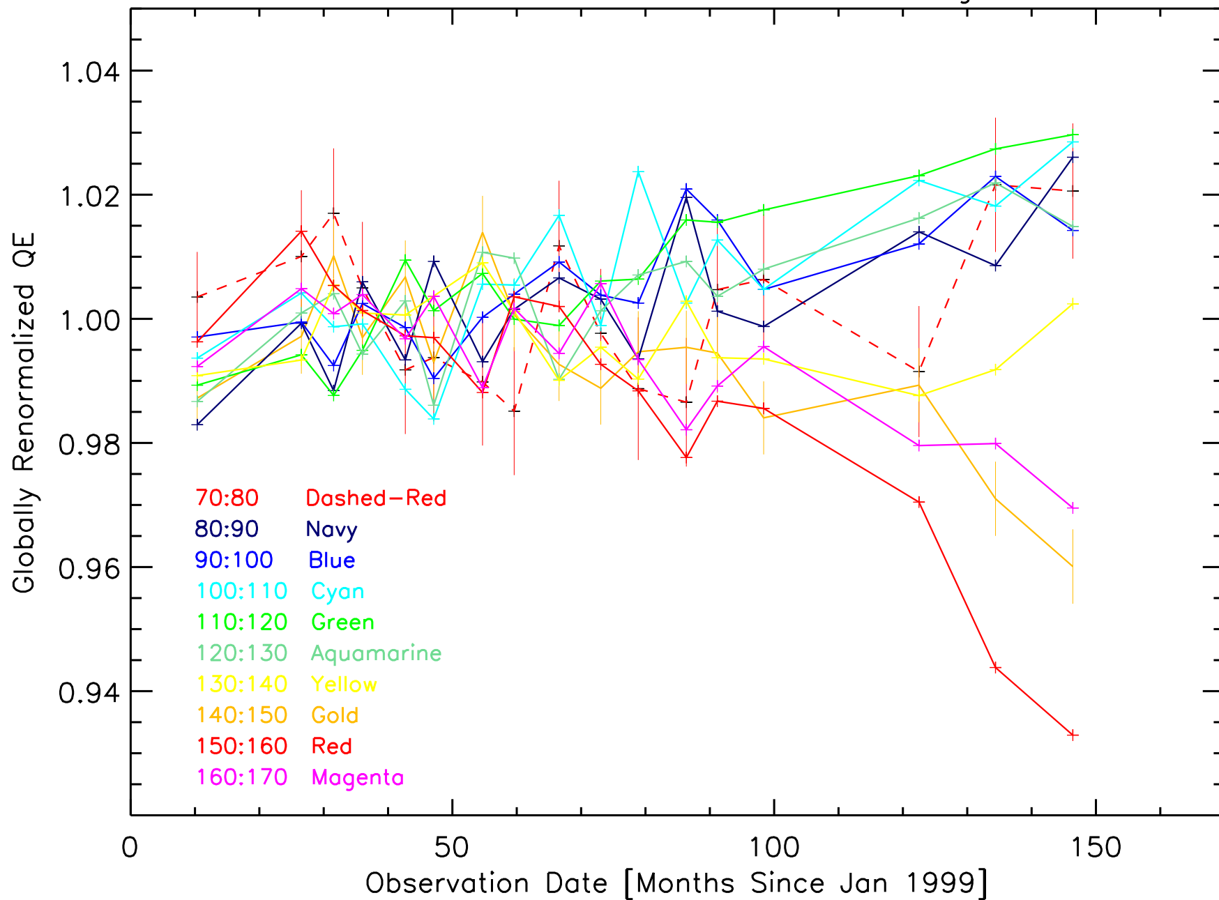
HZ43 Pos-Order Bands 70:80 to 160:170 Angstrom
