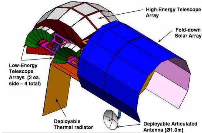
Fig. 1. EXIST on orbit. The 131^\circ \times 65^\circ FoV of the HET array is zenith-oriented with the long direction perpendicular to the orbit velocity vector and “nodded” by \pm 20^\circ every \sim 20 min so that the full sky is scanned each orbit.
