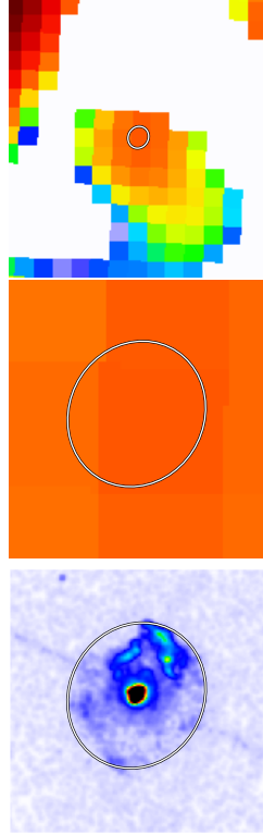
4850 MHz: Radio (4850 MHz continuum)
