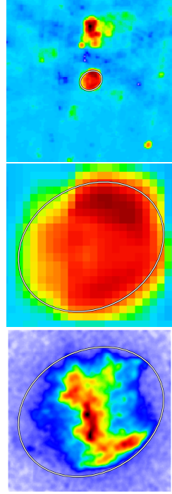
NRAO VLA Sky Survey (NVSS): Radio (1.4 GHz Continuum)
