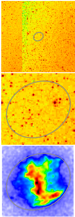
Digitized Sky Survey: Optical (I or E band images with a few exceptions)
