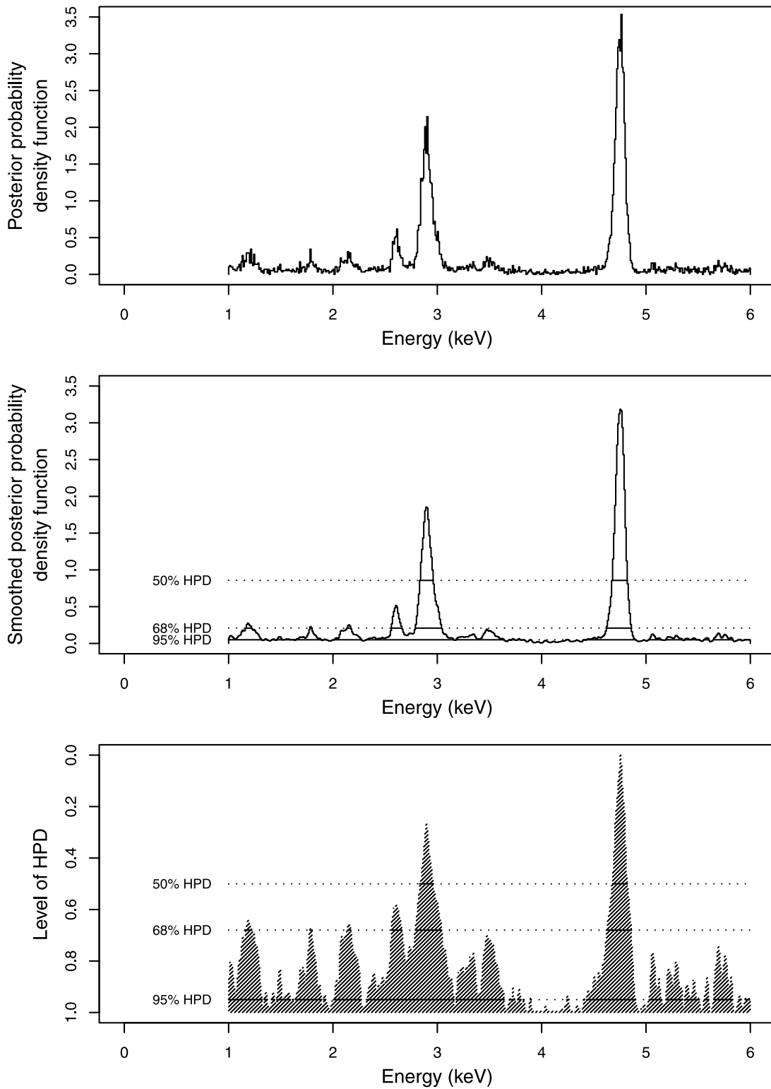
FIG. 3.—Comparing an unsmoothed marginal posterior distribution with its HPD graph computed with Gaussian kernel smoothing. Top: Unsmoothed posterior distribution computed from Monte Carlo draws, plotted with the same resolution as the Chandra energy spectrum. Middle: Posterior distribution smoothed using Gaussian kernel smoothing with standard deviation 0.01 keV, the width of one energy bin in the Chandra spectrum. Based on the smoothed posterior distribution, we compute 100 HPD regions with levels ranging from 1% to 100%. These intervals are plotted against their levels in the HPD graph shown on the bottom. The horizontal solid lines in the middle and bottom panels are the 50%, 68%, and 95% HPD regions, and the horizontal dotted lines are the intervals outside each HPD region.
