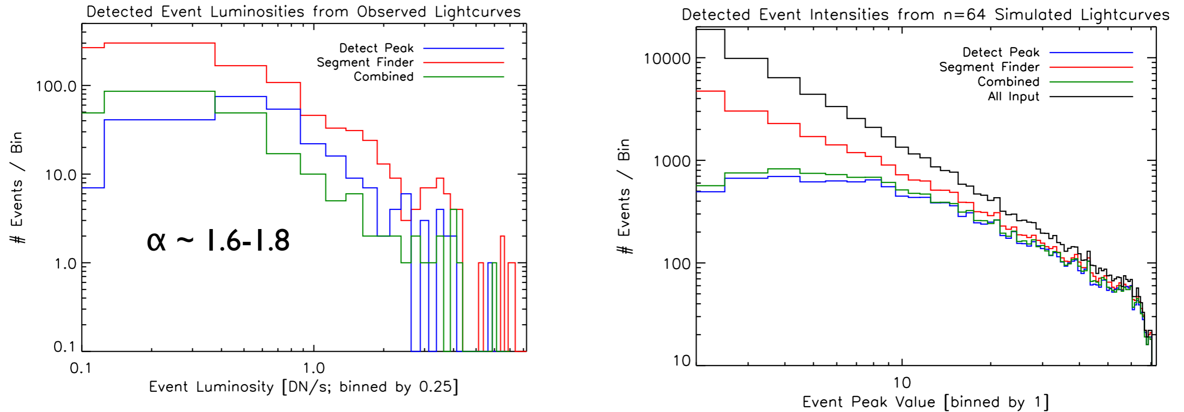
Figure 4 Performance of the algorithms on observed and simulated lightcurves. Left Number versus luminosity (DN/s) of detected events in 15 lightcurves observed with Hinode XRT, with sensitivity parameters in each algorithm set to optimize false positives. Fitting the curves above DN/s = 0.3 gives the following powerlaw index values: 1.81 (Segment Finder), 1.77 (Detect Peak), 1.59 (combined). Right Number versus peak intensity of detected events in 1000 simulated lightcurves, with sensitivity parameters in each algorithm set to optimize false positives. The black line shows the histogram of all peak intensities in the simulated data set. The algorithms perform equally well for bright events, but the probability of detection decreases for weaker events. This decrease is due to a decrease in sensitivity to weak events (for Detect Peak and the combined algorithm), and also because weak events are undetected when they occur over the same time interval as a stronger event.
