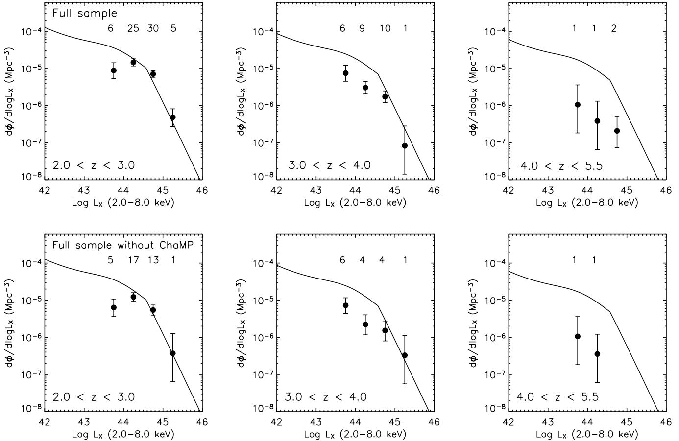
FIG. 12.— Comparison of the high-redshift XLF between the full sample ( top ) and that excluding the ChaMPAGNs ( bottom ). The data points are the same as in Fig. 9. The solid line is the best-fit LDDE model of Ueda et al. (2003) that exemplifies our differences at high redshift. The number of AGNs per luminosity and redshift bin is shown above their respective data point.
