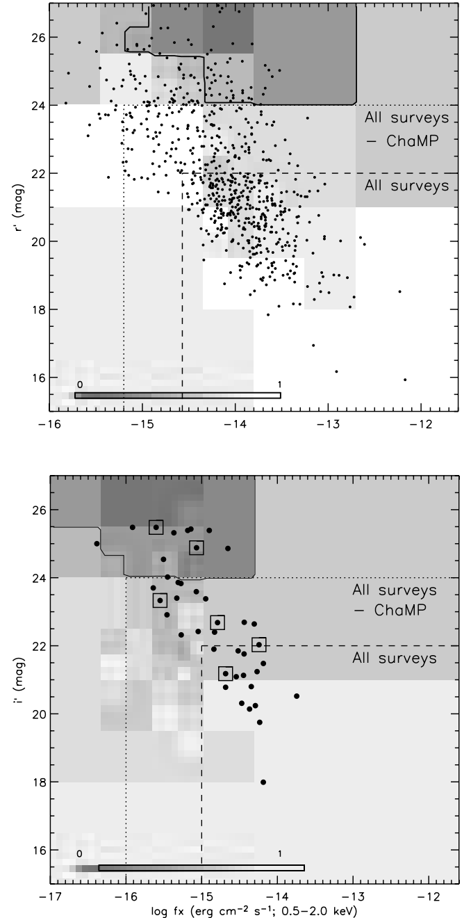
Fig. 2.— Fraction of identified (i.e., redshift is known) sources as a function of X-ray and optical flux in the hard/ r' ( top ) and soft/ i' ( bottom ) energy bands. The gray-scale image ranges from zero ( darkest ) to 100% ( lightest ) of sources having redshifts mainly from optical spectroscopy. The AGNs are shown with a filled circle in the hard map for those at z < 3 and soft map for those at z > 3 . In the soft-band map, those AGNs at z > 4 are also marked by a square. The X-ray and optical flux limits for our analysis are shown by the dashed and dotted lines, respectively. Since the ChaMP survey has a reasonable degree of completeness only at brighter flux levels, we only include ChaMP AGNs that fall in the lower right region as defined by the dashed lines. The faintest limits ( dotted line ) are determined by the fraction of identified sources ( > 50\% ).
